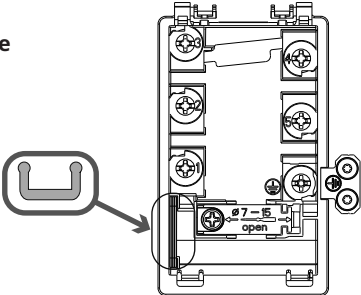
380 - 415V ~ 2+N+GND
