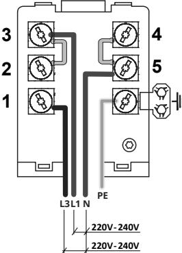
380 - 415V ~ 2+N+GND
