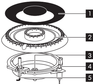
1 Burner cap
