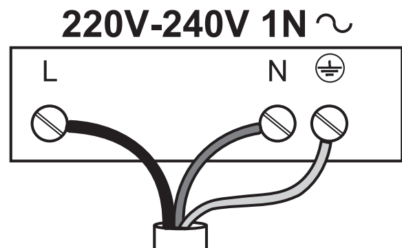
Connection diagram
